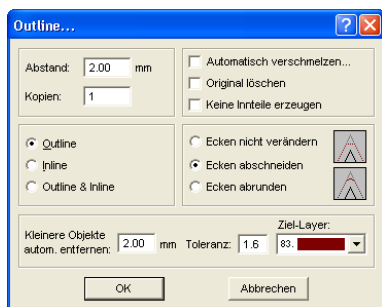
Abb. 4.6-6: Outline-Dialog
